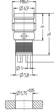
ESGP_soldering-contact
