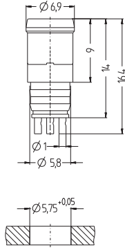
ESHP_soldering-contact
