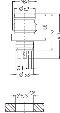
SESP_soldering-contact
